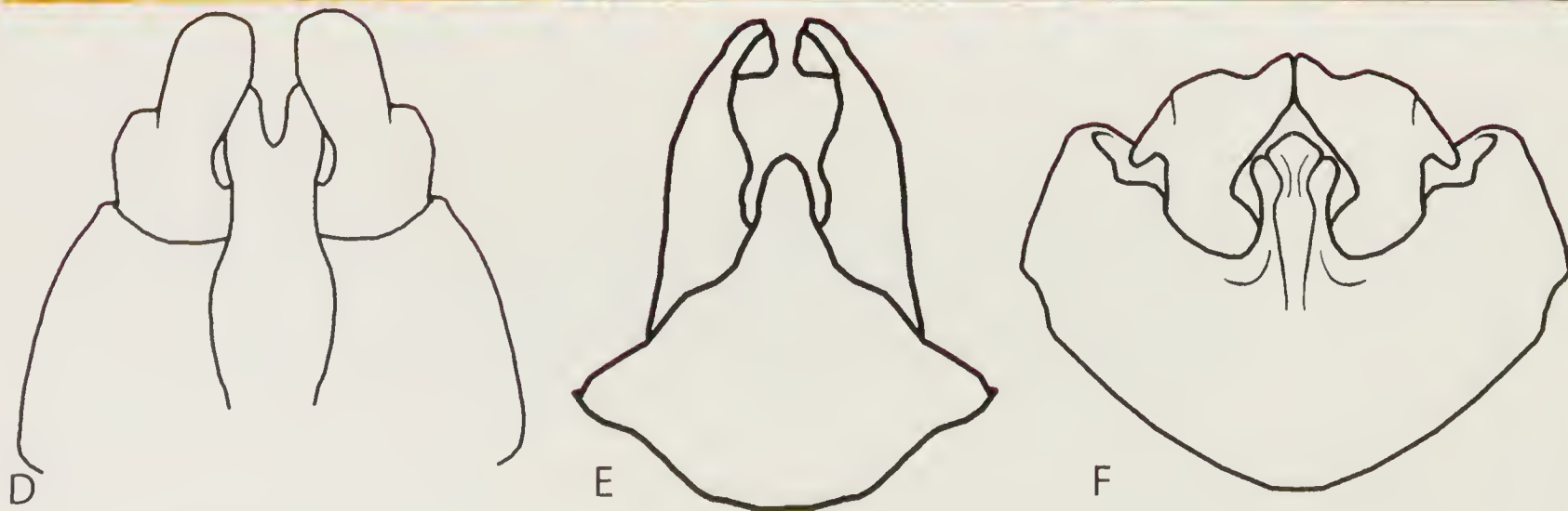
Figure 7. Male terminalia of Achilidae, ventral view. A, D. Catonia picta ; B, E. Synechdoche dimidiata ; C, F. Opsiplanon luellus .
